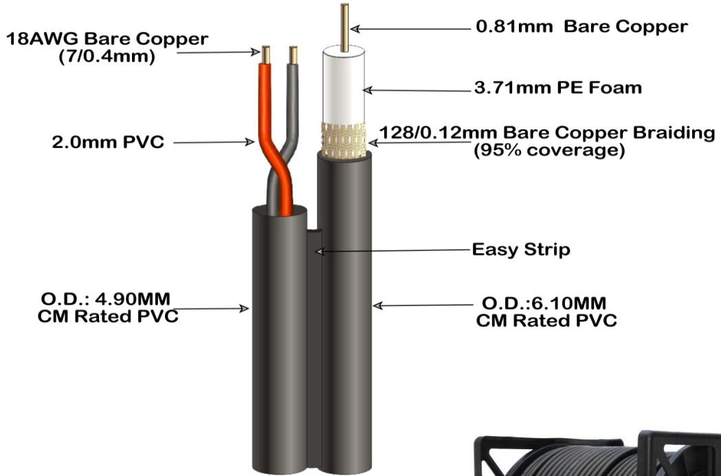
Bare Copper conductor Siamese Cable
